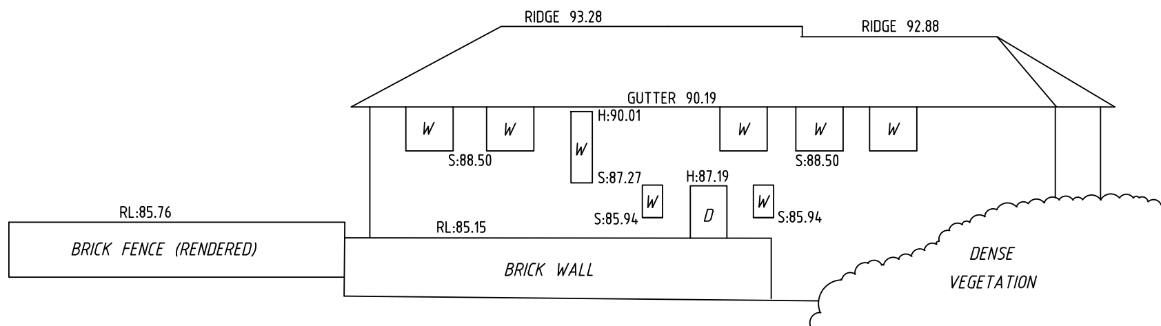
SOUTH-WESTERN ELEVATION No.15 AMAROO AVENUE
