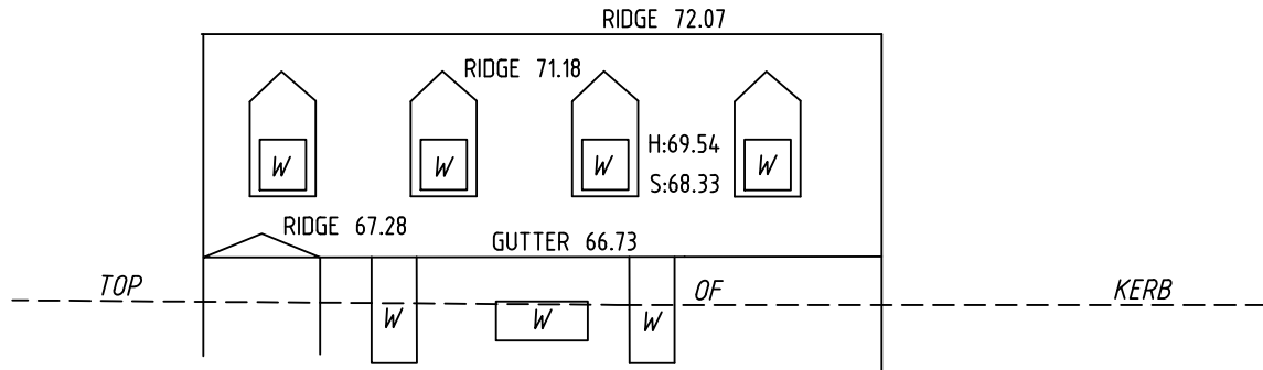
NORTH-EASTERN ELEVATION No.119 DEEPWATER ROAD
