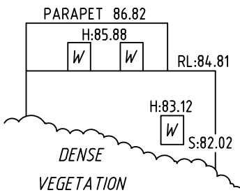
NORTH-WESTERN ELEVATION No.78 DEEPWATER ROAD
