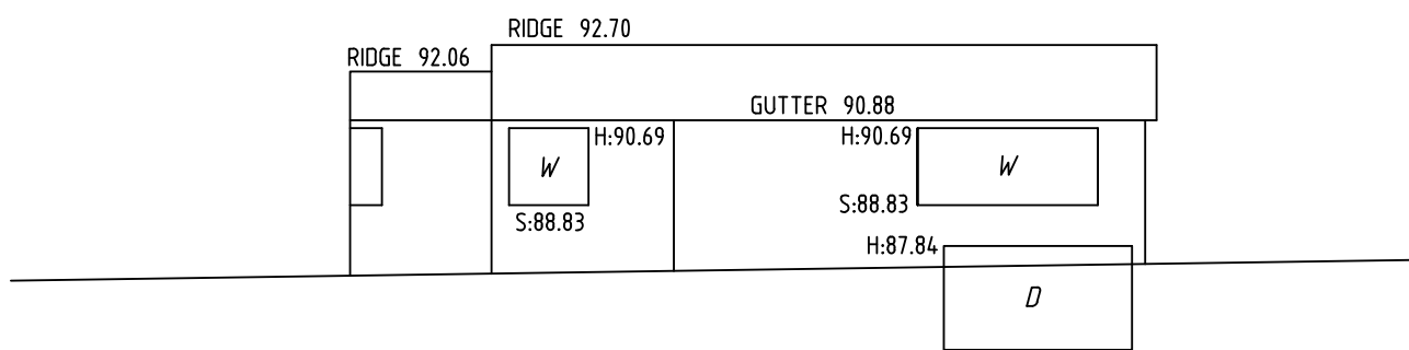
EASTERN ELEVATION No.13 AMAROO AVENUE
