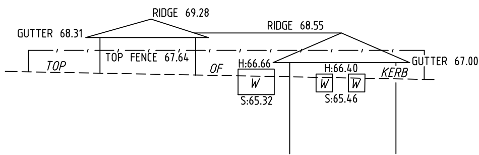
NORTH-EASTERN ELEVATION No.109 DEEPWATER ROAD
