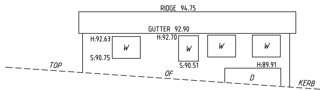
WESTERN ELEVATION No.6 AMAROO AVENUE
