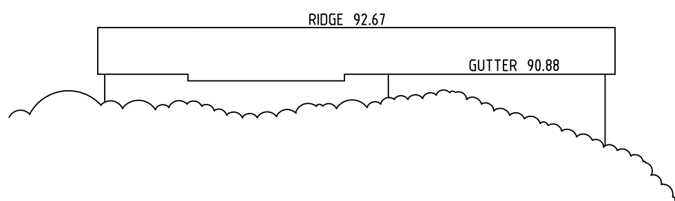
WESTERN ELEVATION No.13 AMAROO AVENUE
