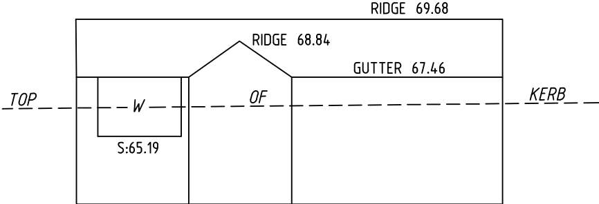
NORTH-EASTERN ELEVATION No.111 DEEPWATER ROAD
