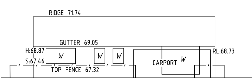
NORTH-EASTERN ELEVATION No.113 DEEPWATER ROAD
