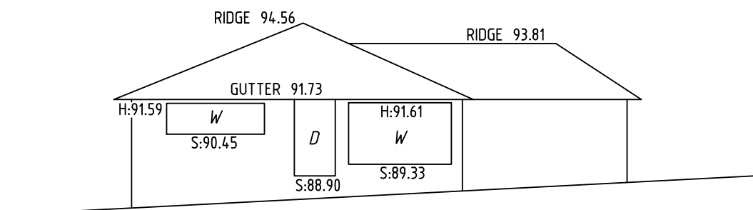
EASTERN ELEVATION No.11 AMAROO AVENUE
