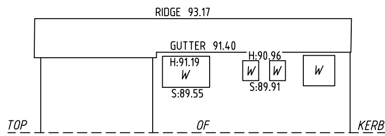
WESTERN ELEVATION No.10 AMAROO AVENUE
