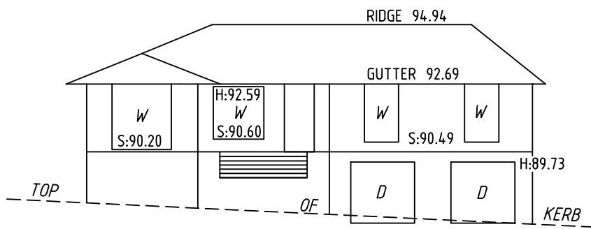
WESTERN ELEVATION No.8 AMAROO AVENUE
