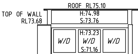
NORTHERN ELEVATION No.76 DEEPWATER ROAD
